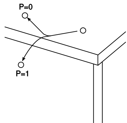
q / The marble has zero probability of being reflected from the edge of the table. (This example has U < 0 , not U > 0 as in figures p and r).
